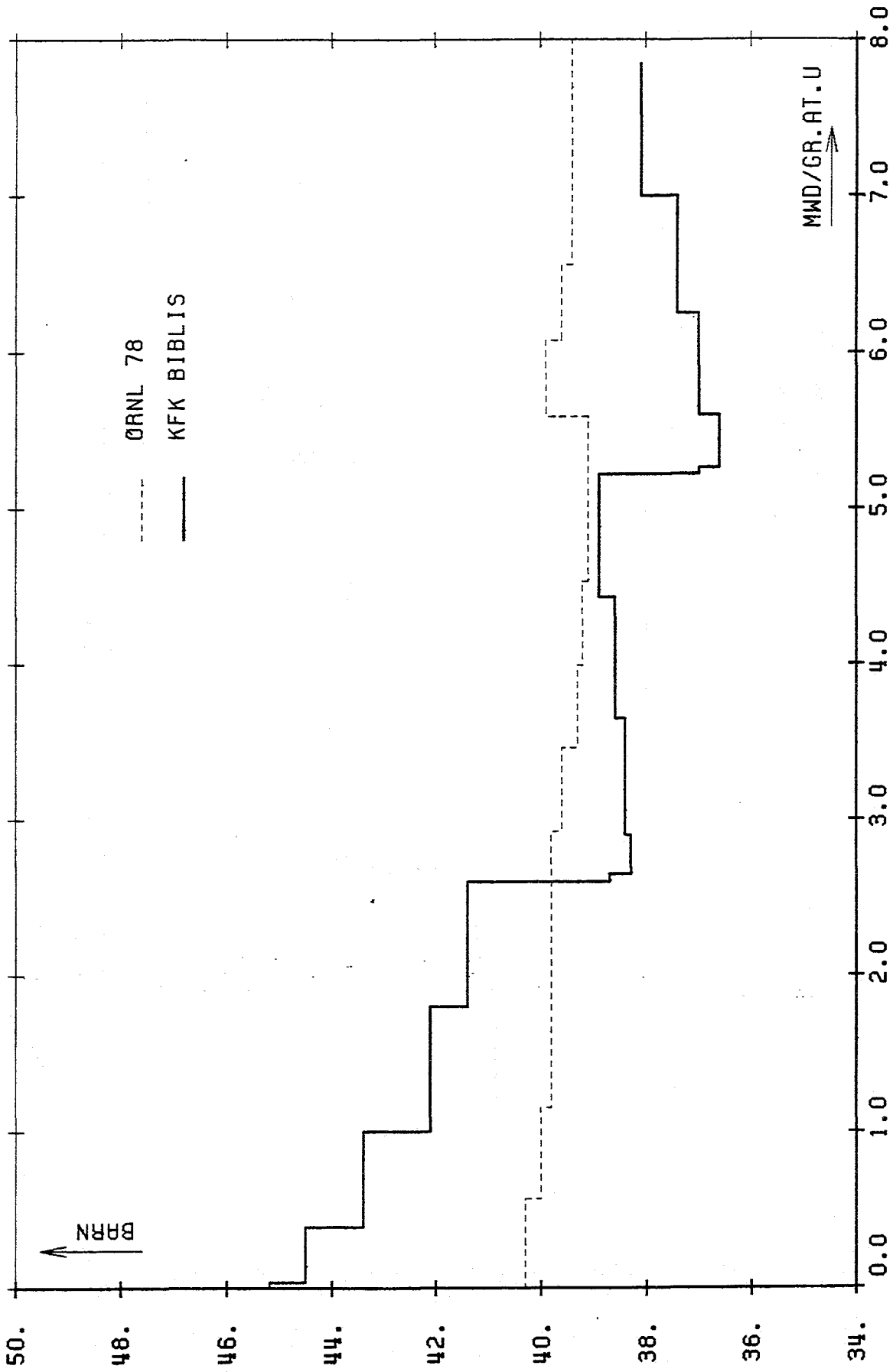
Abb. C.2-7 PU241 SCAPT
