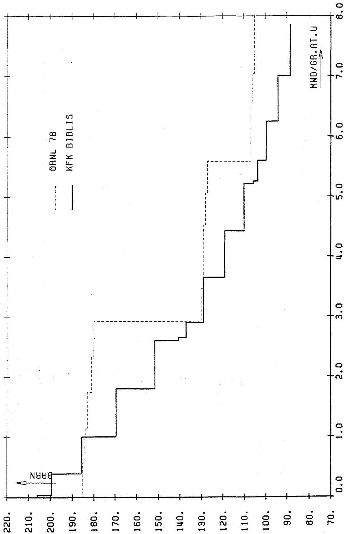
Abb. C. 2-6 PU240 SCAPT
